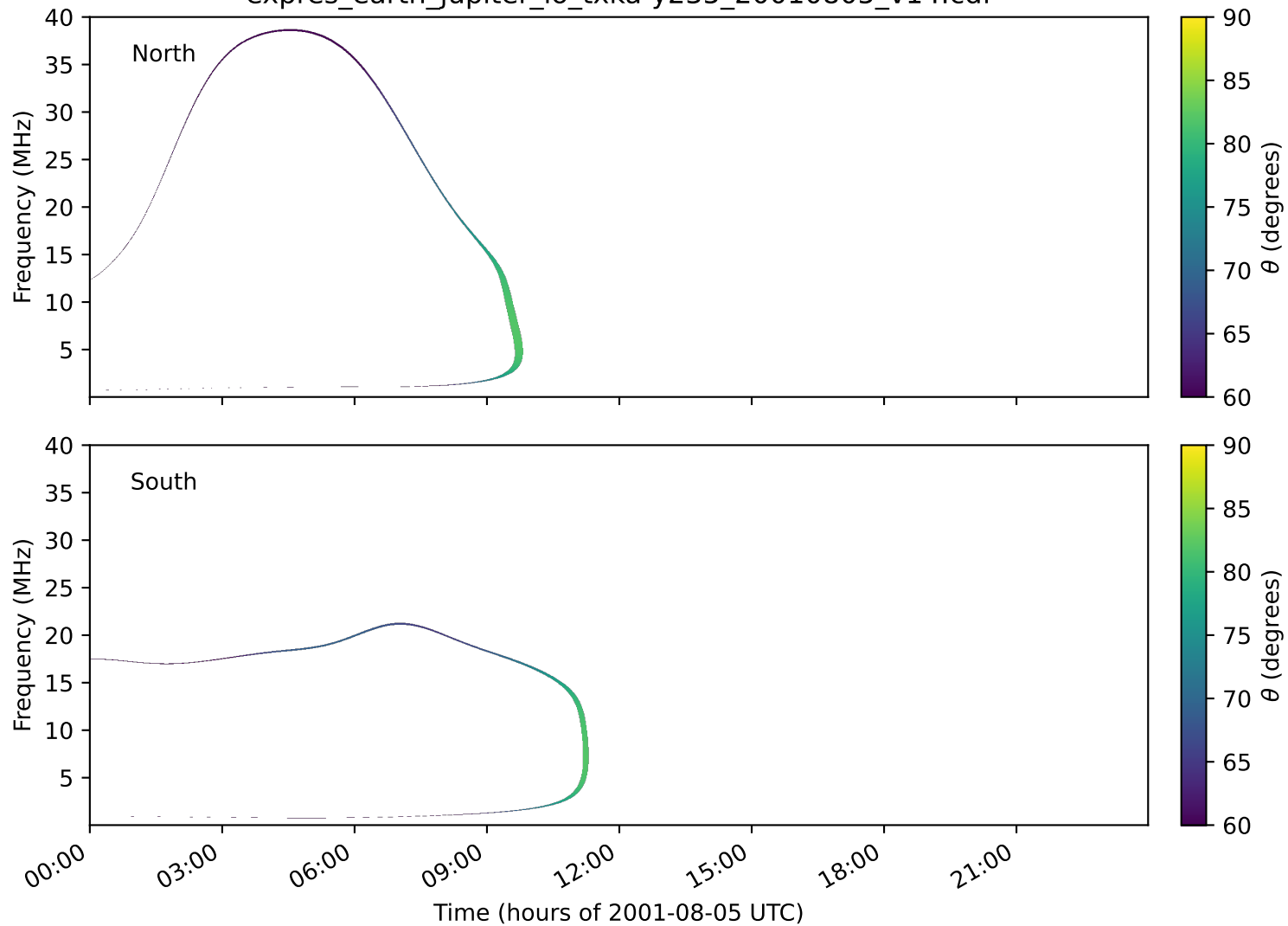
expres_earth_jupiter_io_txka-y235_20010805_v14.cdf
