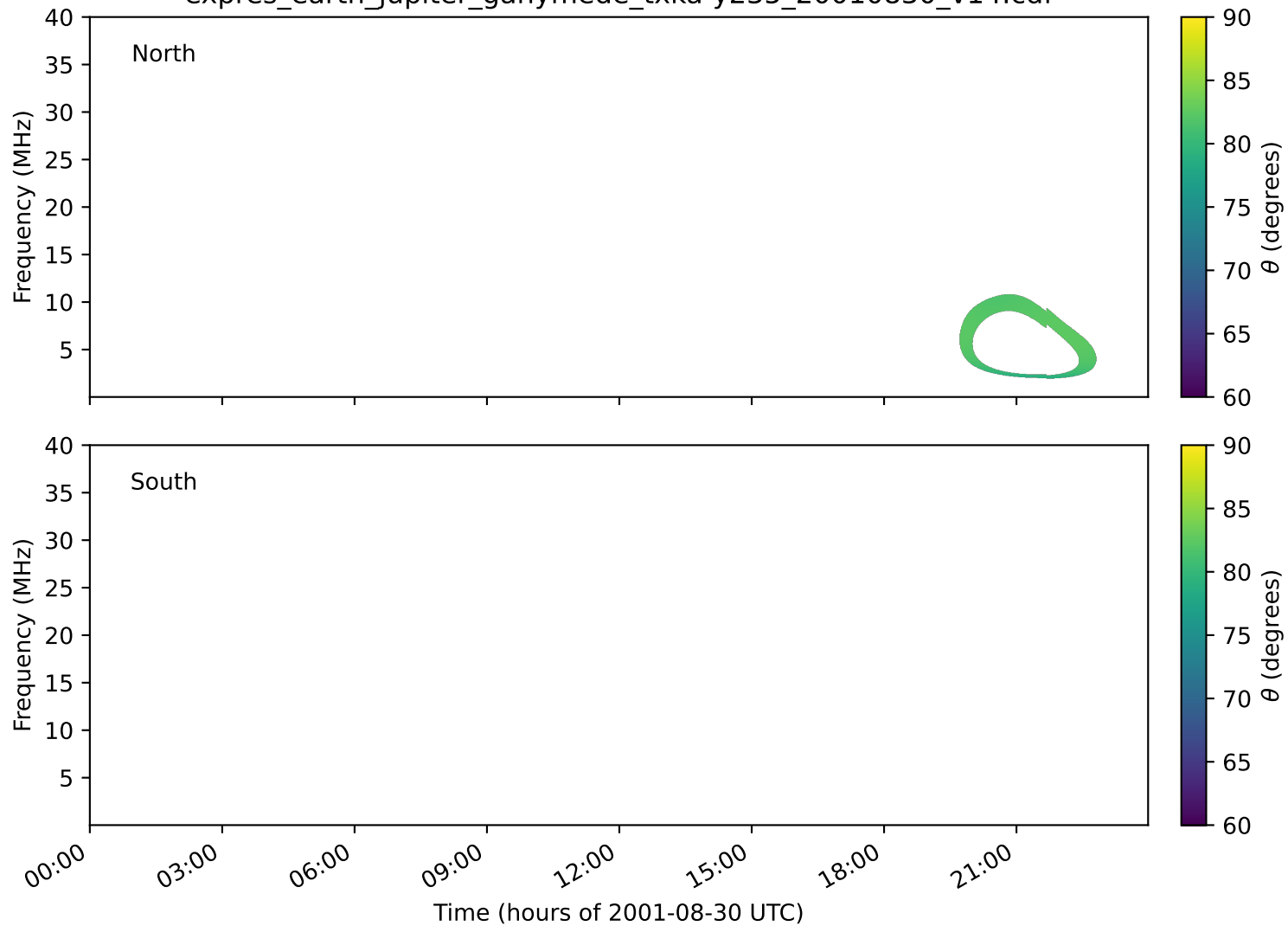
expres_earth_jupiter_ganymede_txka-y235_20010830_v14.cdf
