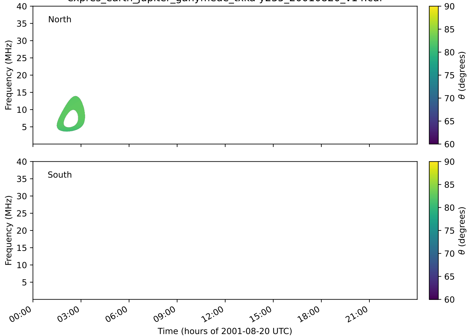
expres_earth_jupiter_ganymede_txka-y235_20010820_v14.cdf
