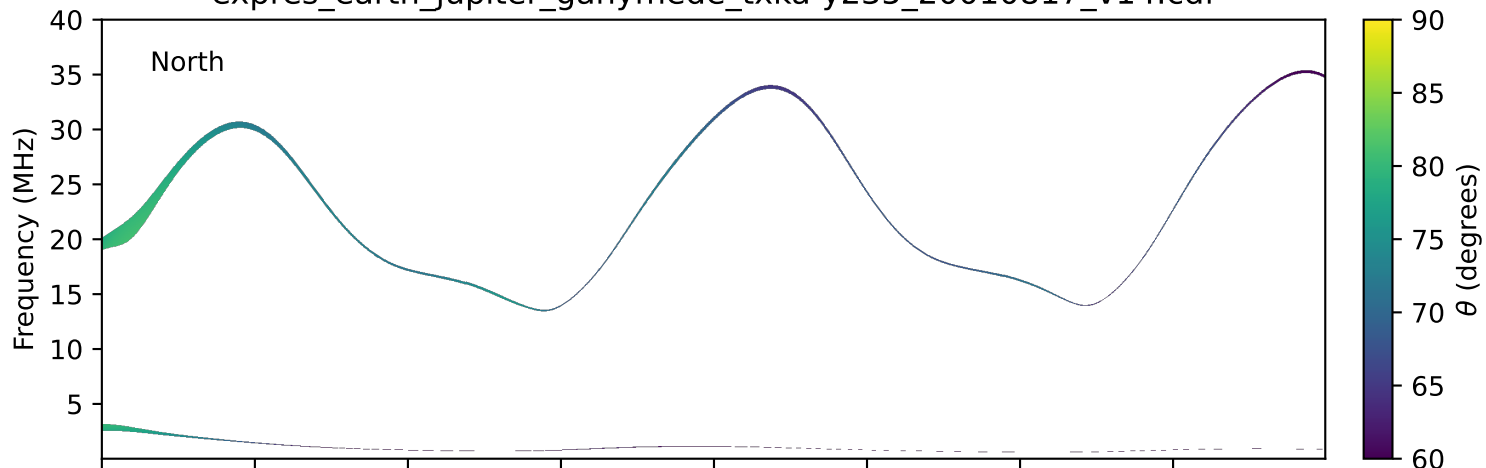
expres_earth_jupiter_ganymede_txka-y235_20010817_v14.cdf
