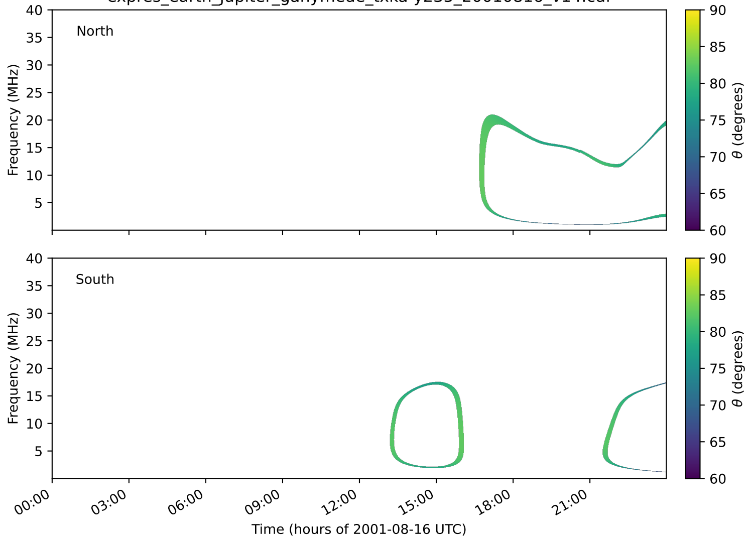
expres_earth_jupiter_ganymede_txka-y235_20010816_v14.cdf
