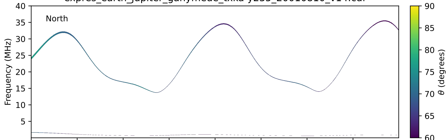
expres_earth_jupiter_ganymede_txka-y235_20010810_v14.cdf
