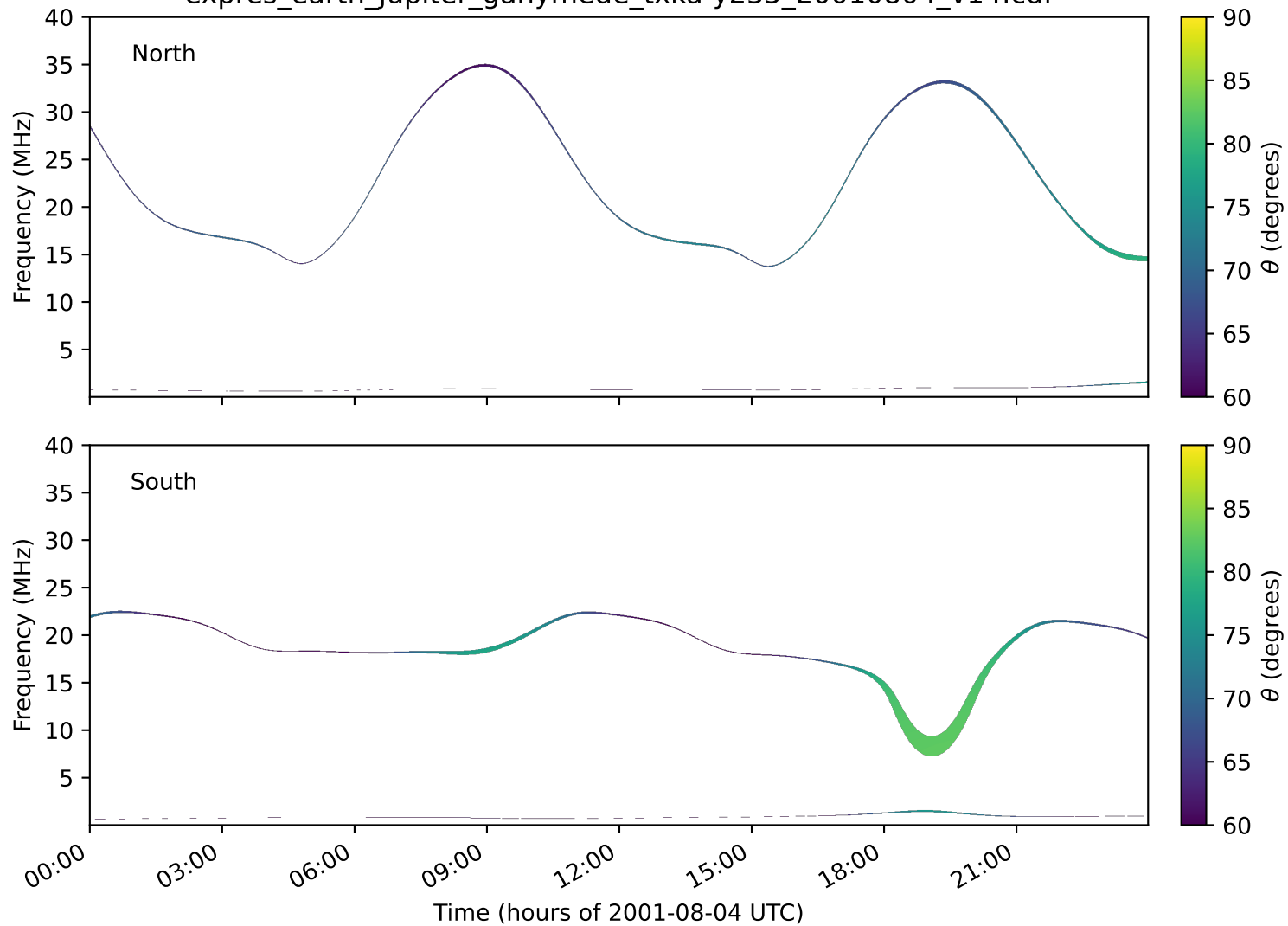
expres_earth_jupiter_ganymede_txka-y235_20010804_v14.cdf
