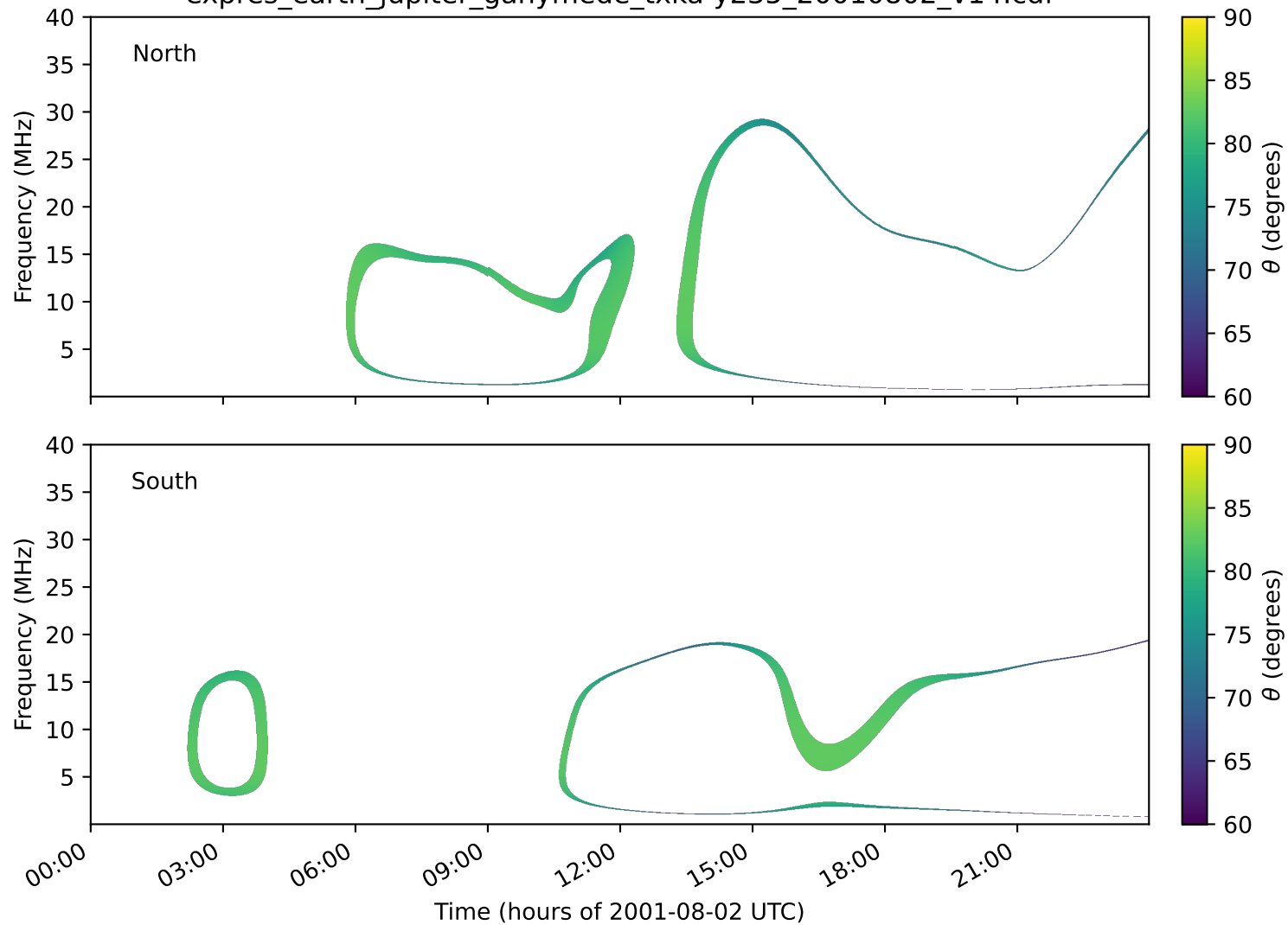
expres_earth_jupiter_ganymede_txka-y235_20010802_v14.cdf
