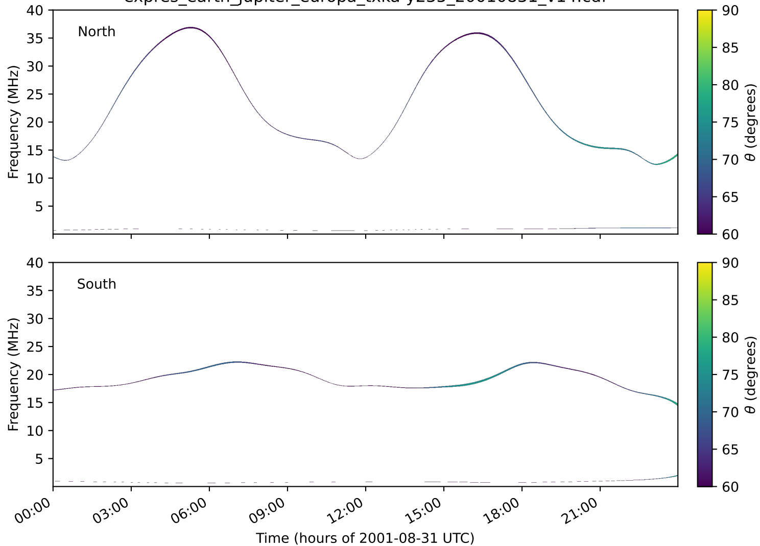
expres_earth_jupiter_europa_txka-y235_20010831_v14.cdf
