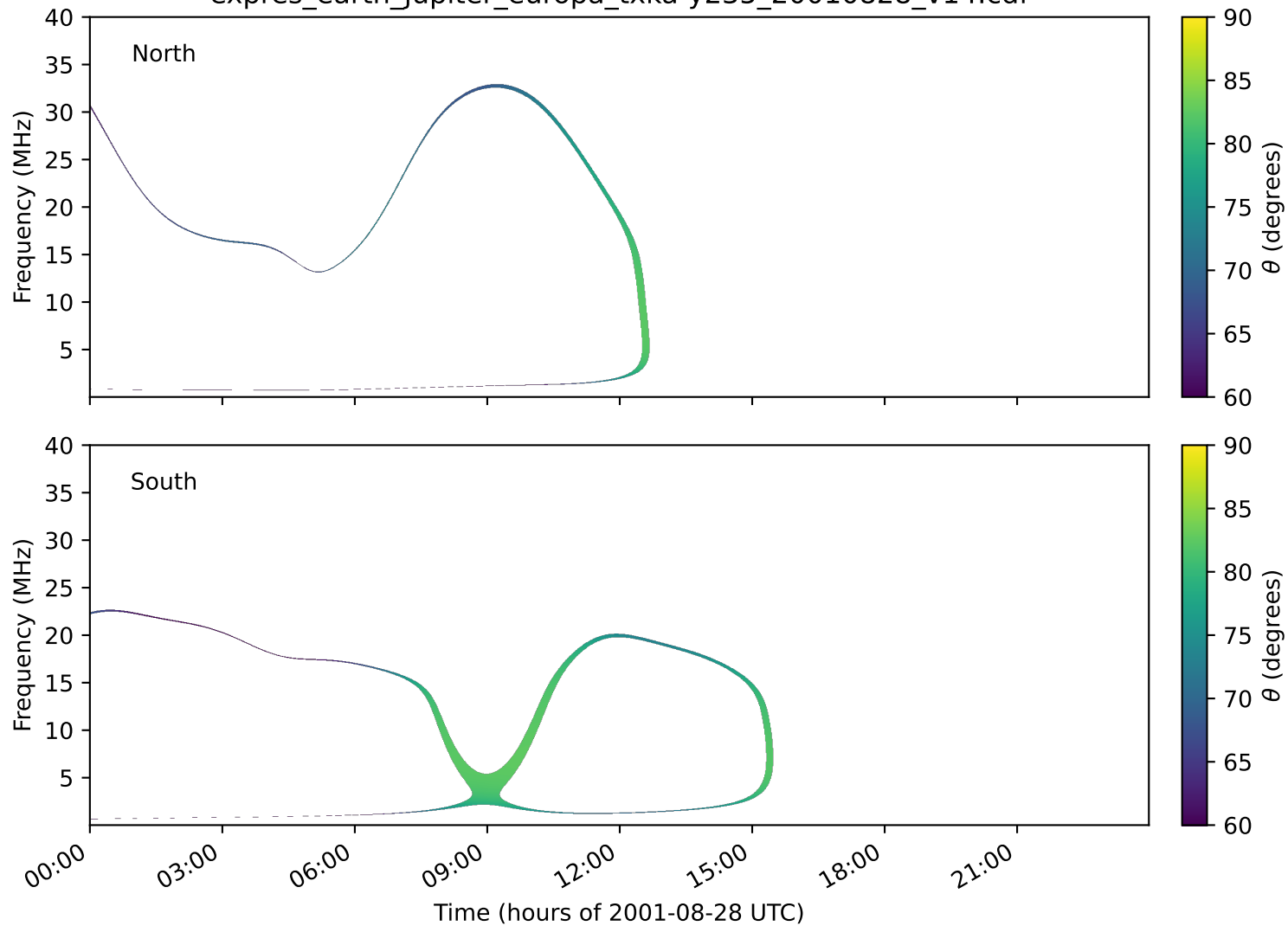
expres_earth_jupiter_europa_txka-y235_20010828_v14.cdf
