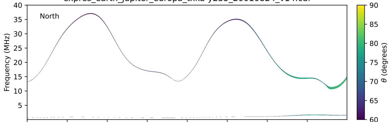
expres_earth_jupiter_europa_txka-y235_20010824_v14.cdf
