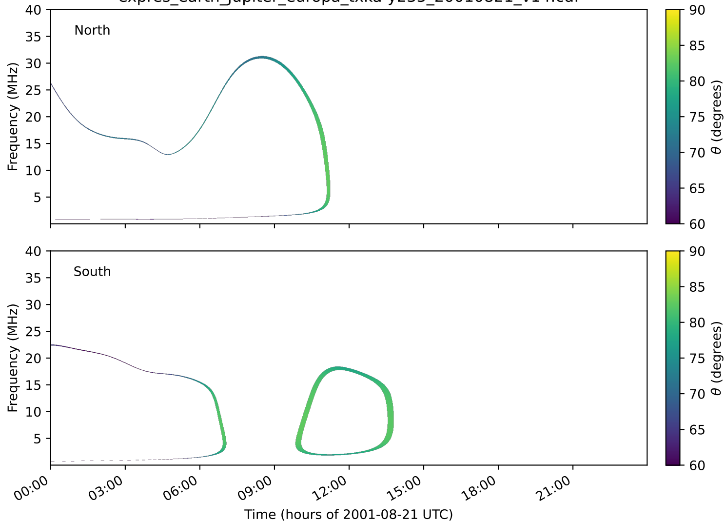
expres_earth_jupiter_europa_txka-y235_20010821_v14.cdf
