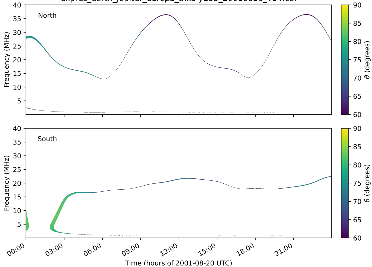
expres_earth_jupiter_europa_txka-y235_20010820_v14.cdf
