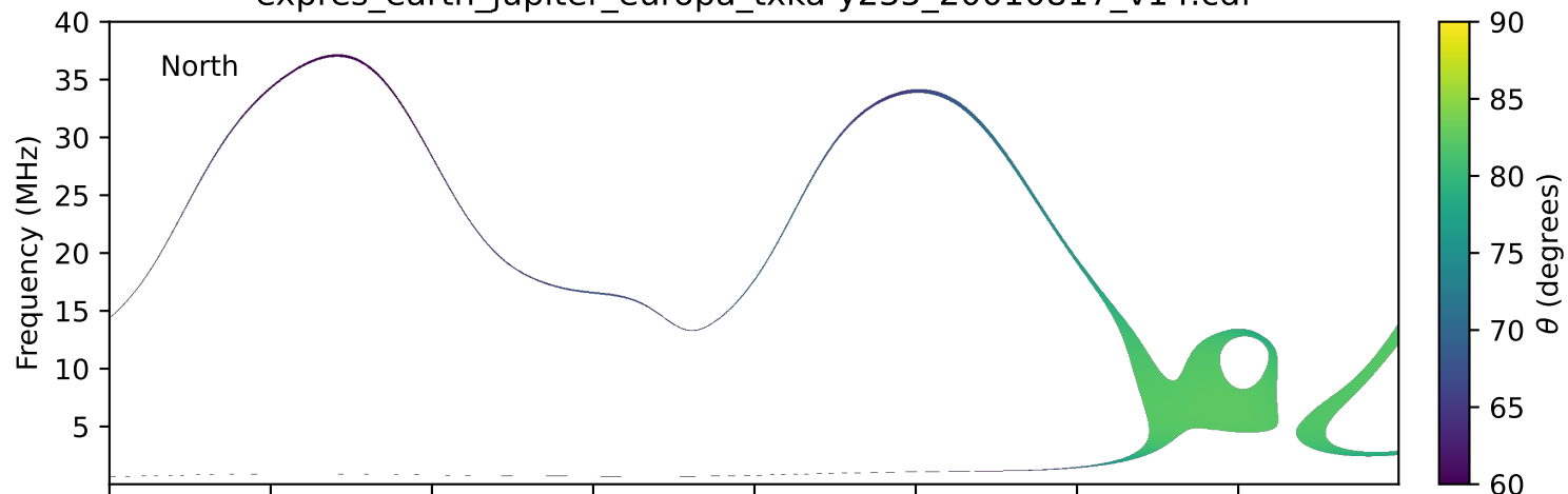
expres_earth_jupiter_europa_txka-y235_20010817_v14.cdf
