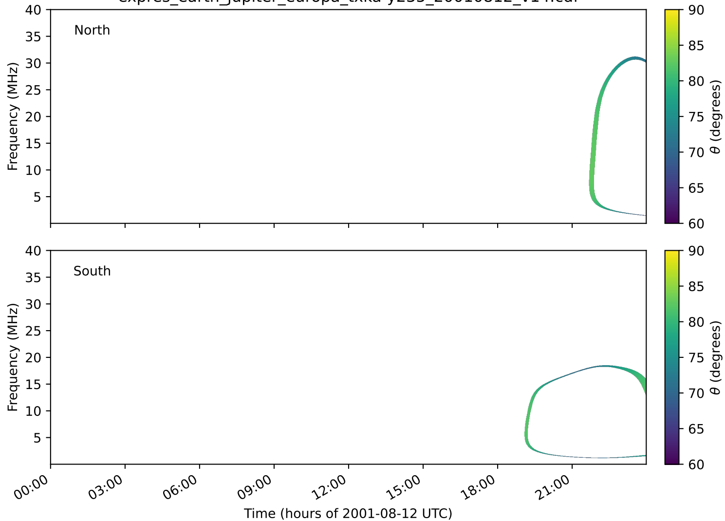
expres_earth_jupiter_europa_txka-y235_20010812_v14.cdf
