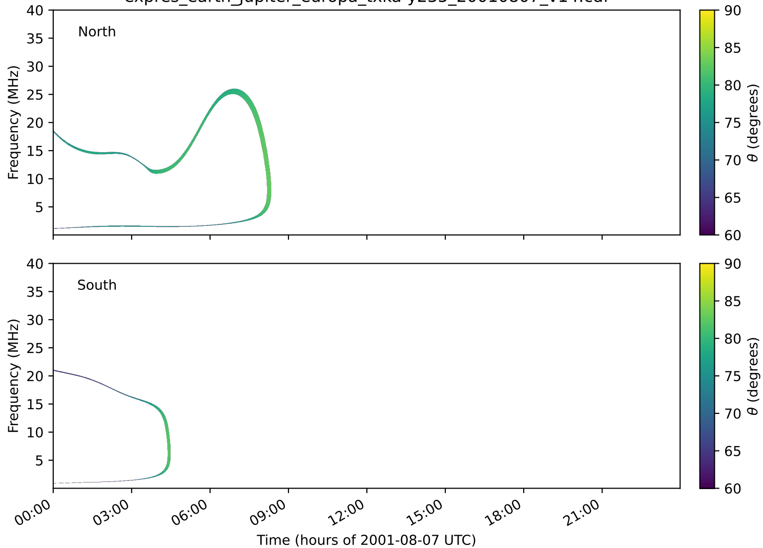
expres_earth_jupiter_europa_txka-y235_20010807_v14.cdf
