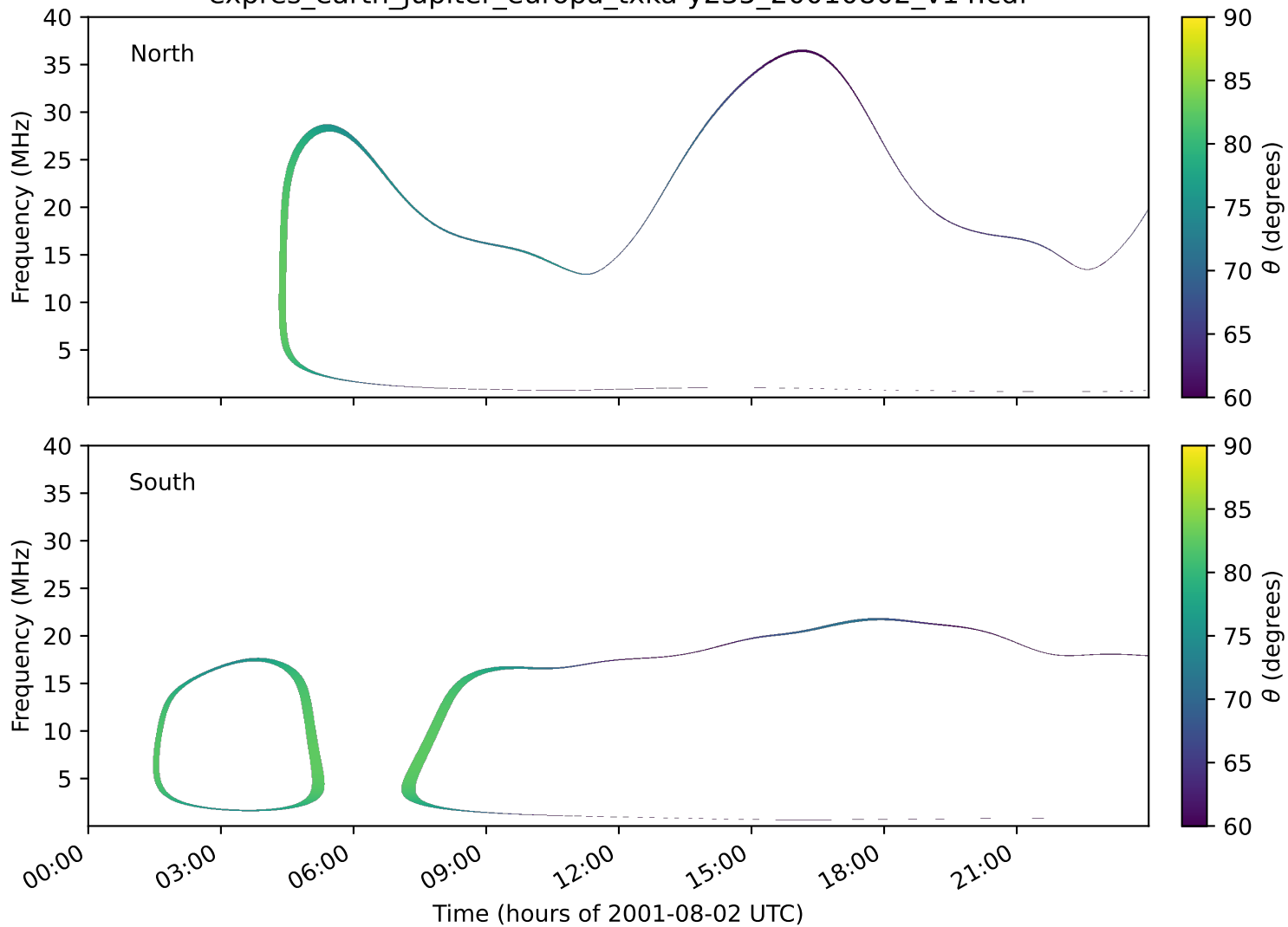
expres_earth_jupiter_europa_txka-y235_20010802_v14.cdf
