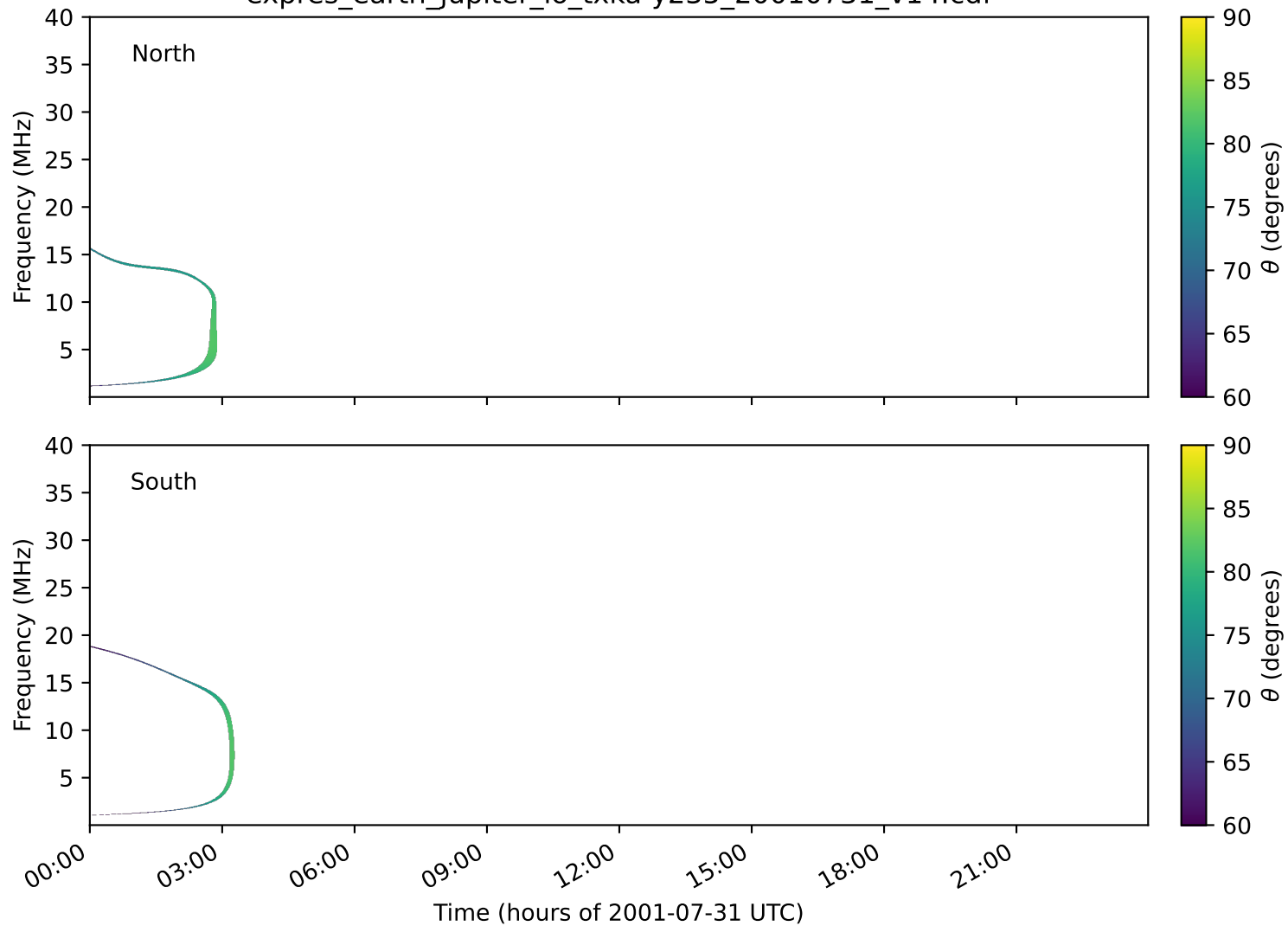
expres_earth_jupiter_io_txka-y235_20010731_v14.cdf
