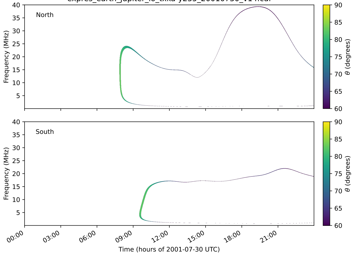
expres_earth_jupiter_io_txka-y235_20010730_v14.cdf
