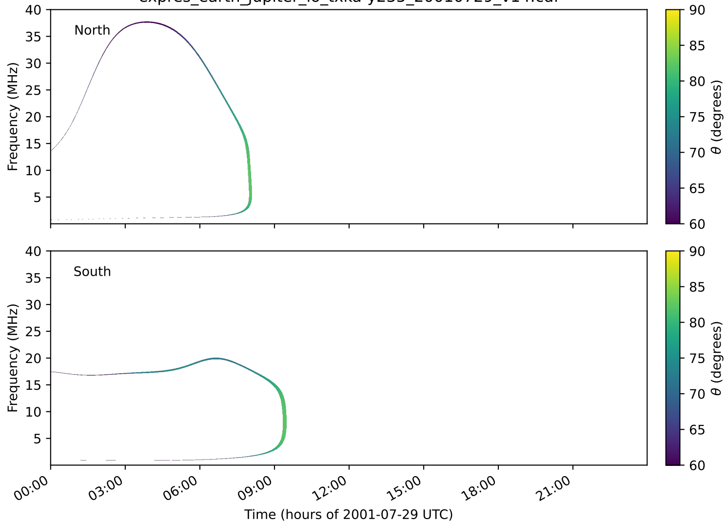
expres_earth_jupiter_io_txka-y235_20010729_v14.cdf
