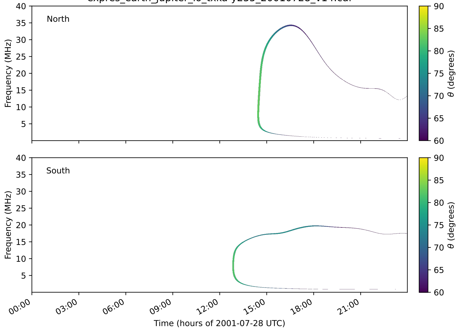
expres_earth_jupiter_io_txka-y235_20010728_v14.cdf
