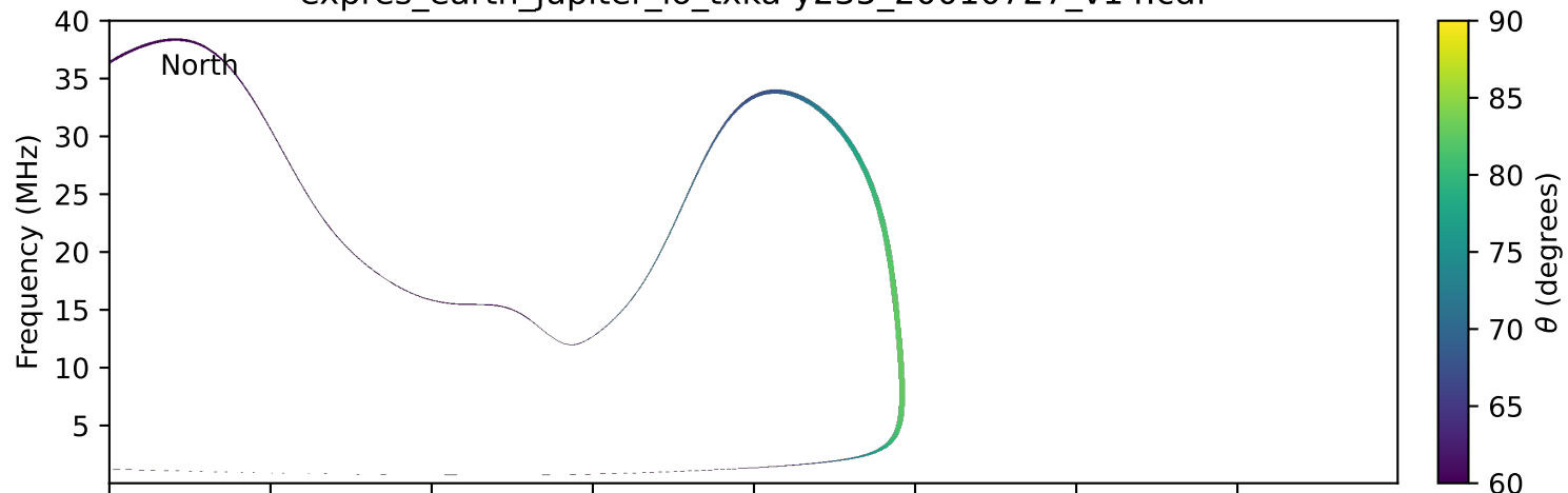
expres_earth_jupiter_io_txka-y235_20010727_v14.cdf
