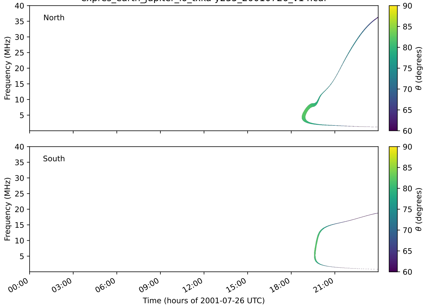
expres_earth_jupiter_io_txka-y235_20010726_v14.cdf
