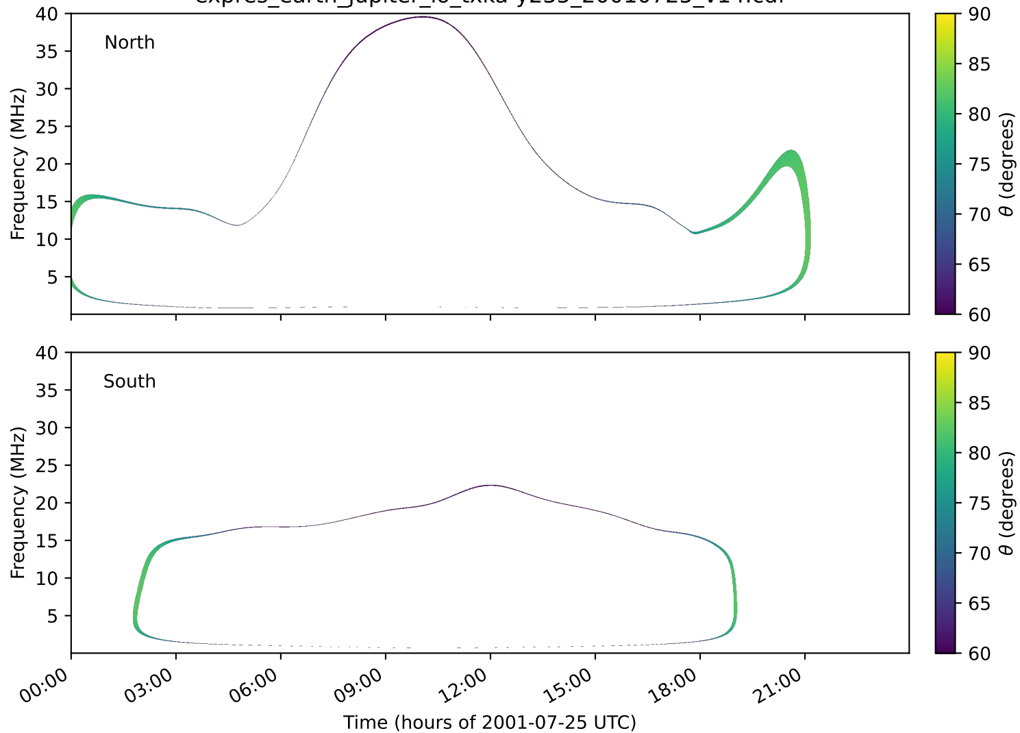
expres_earth_jupiter_io_txka-y235_20010725_v14.cdf
