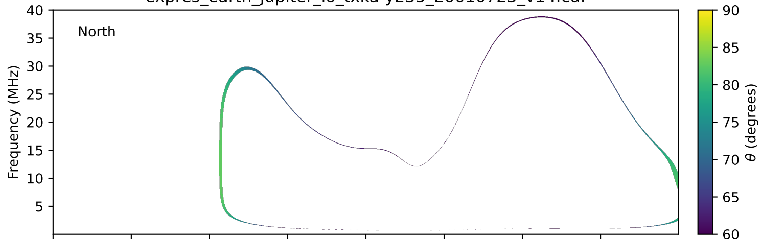
expres_earth_jupiter_io_txka-y235_20010723_v14.cdf
