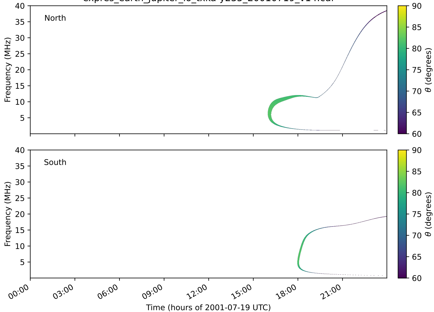
expres_earth_jupiter_io_txka-y235_20010719_v14.cdf
