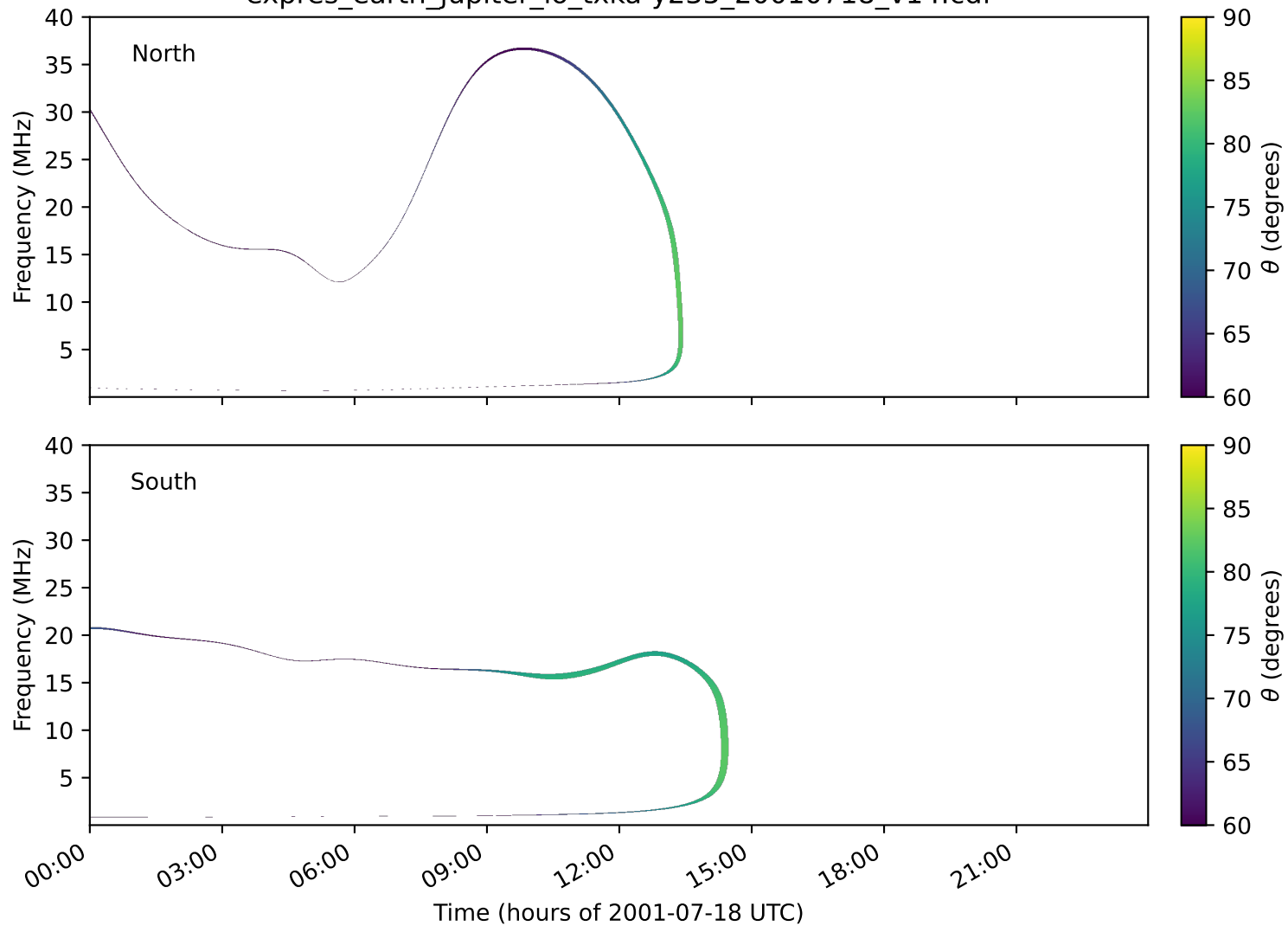
expres_earth_jupiter_io_txka-y235_20010718_v14.cdf
