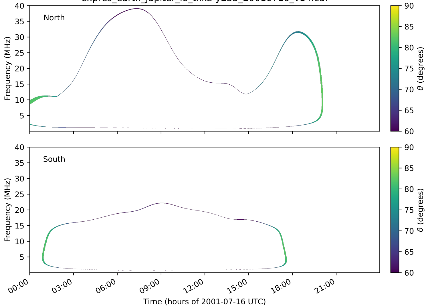
expres_earth_jupiter_io_txka-y235_20010716_v14.cdf
