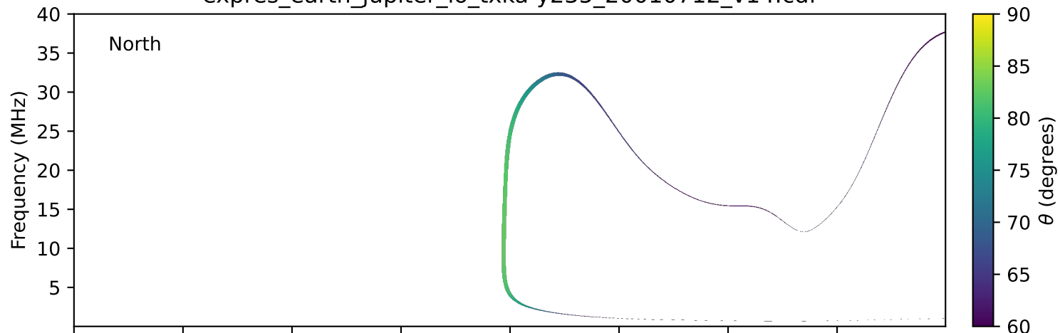
expres_earth_jupiter_io_txka-y235_20010712_v14.cdf
