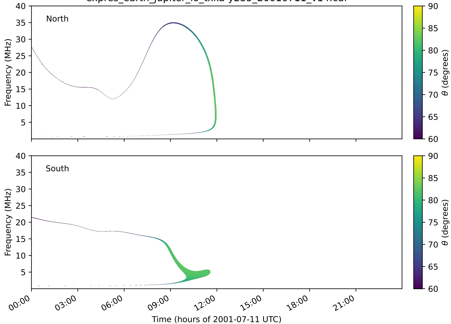
expres_earth_jupiter_io_txka-y235_20010711_v14.cdf
