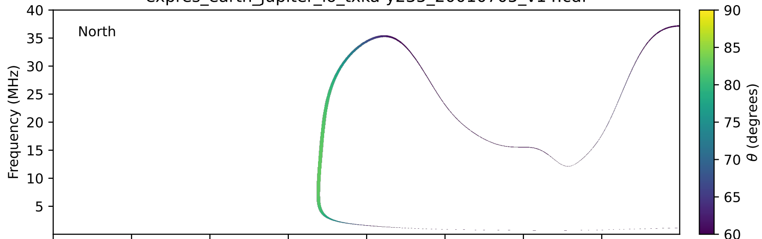
expres_earth_jupiter_io_txka-y235_20010705_v14.cdf
