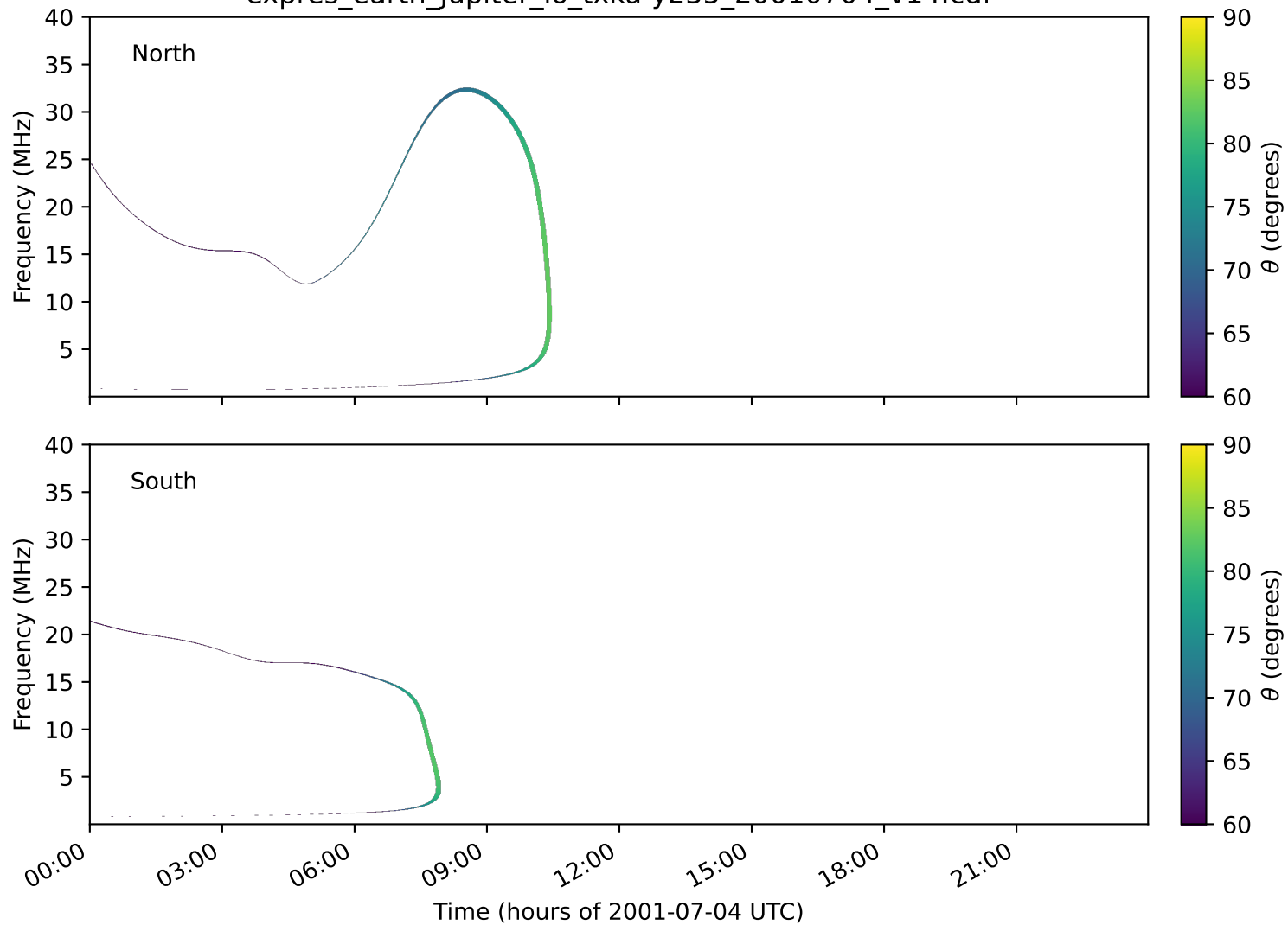
expres_earth_jupiter_io_txka-y235_20010704_v14.cdf
