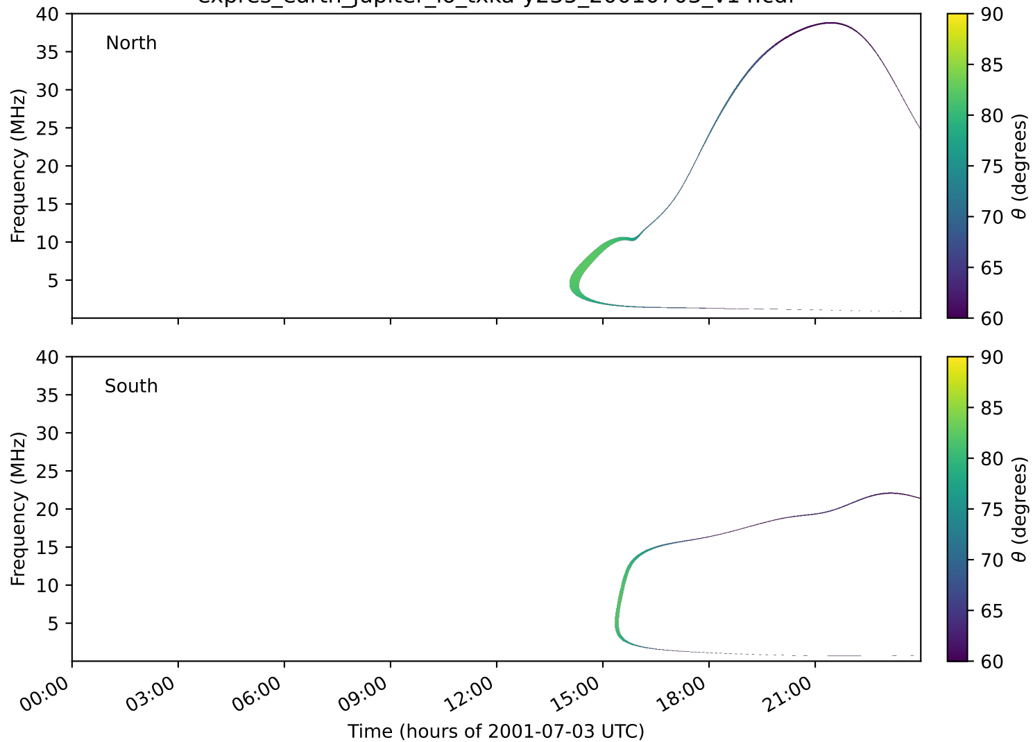
expres_earth_jupiter_io_txka-y235_20010703_v14.cdf
