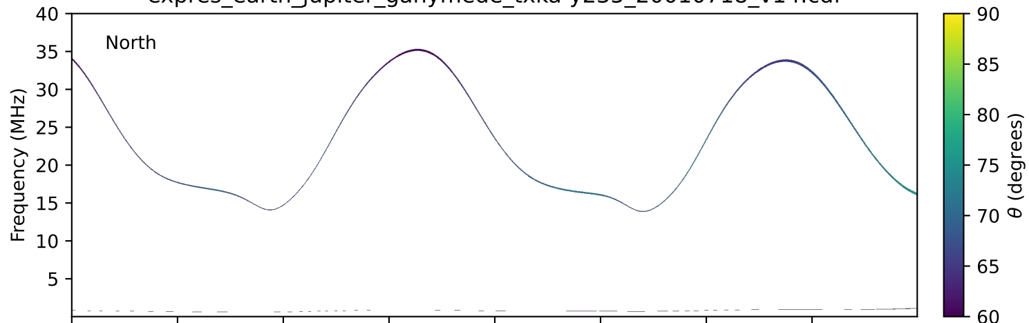
expres_earth_jupiter_ganymede_txka-y235_20010718_v14.cdf
