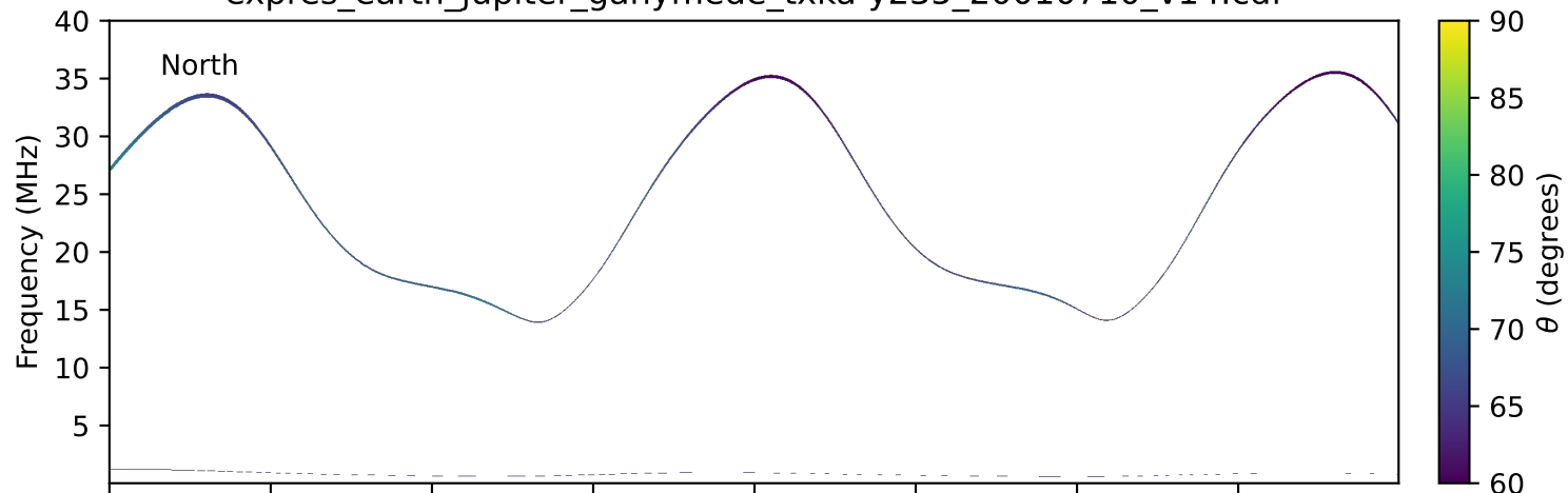
expres_earth_jupiter_ganymede_txka-y235_20010710_v14.cdf
