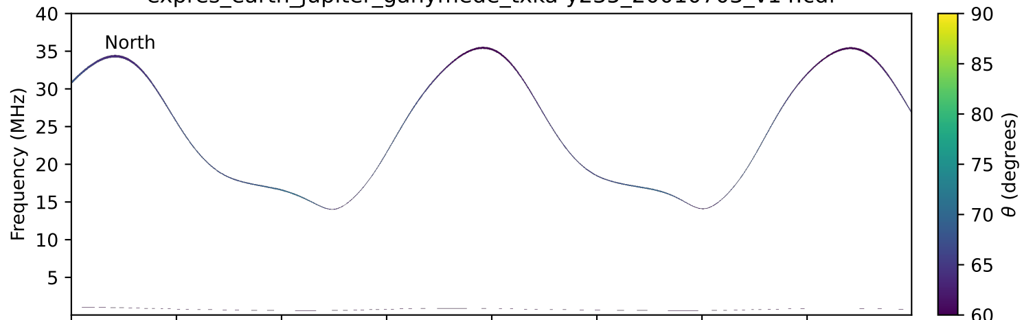
expres_earth_jupiter_ganymede_txka-y235_20010703_v14.cdf
