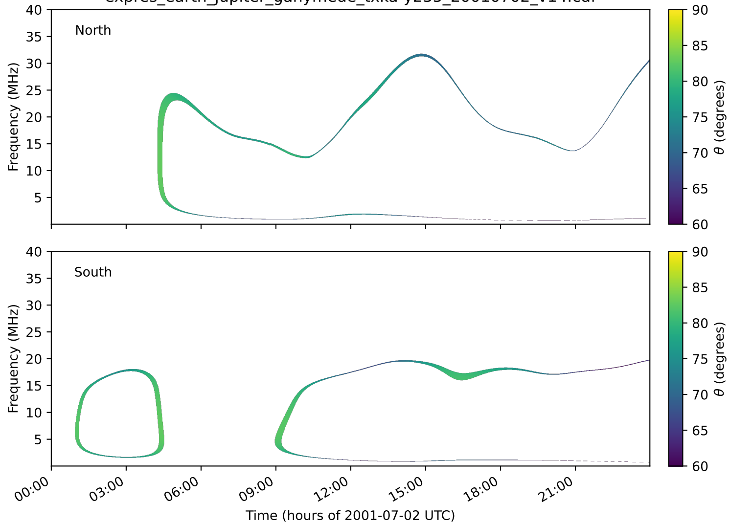
expres_earth_jupiter_ganymede_txka-y235_20010702_v14.cdf
