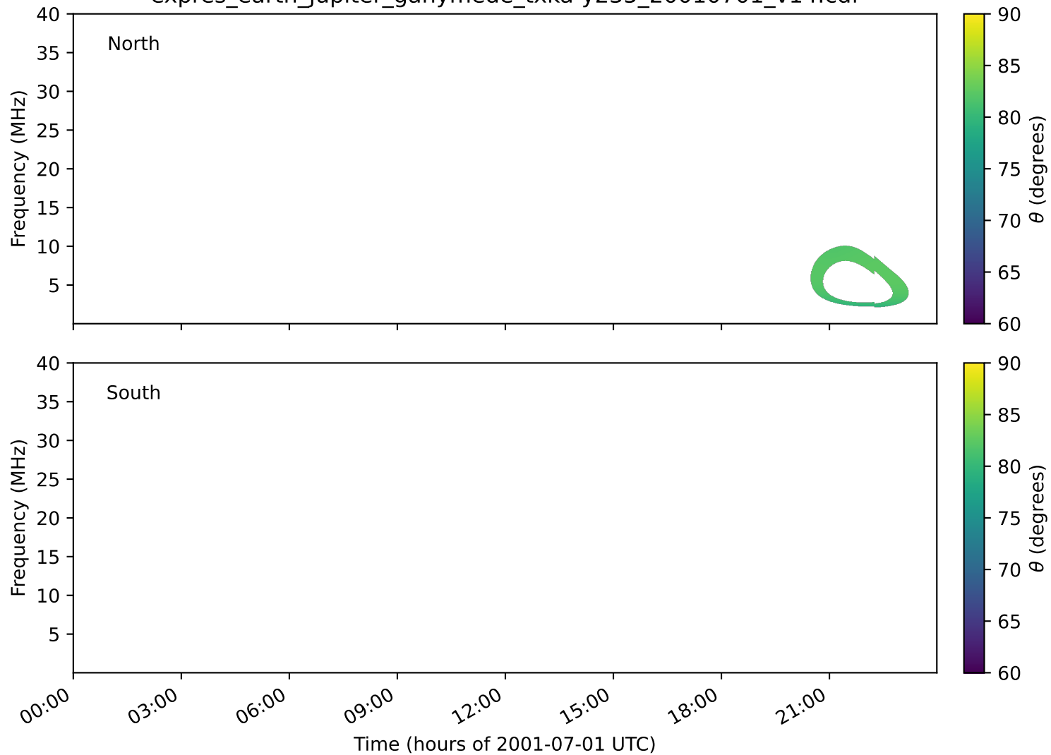
expres_earth_jupiter_ganymede_txka-y235_20010701_v14.cdf
