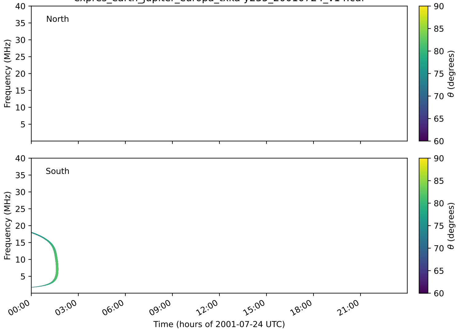
expres_earth_jupiter_europa_txka-y235_20010724_v14.cdf
