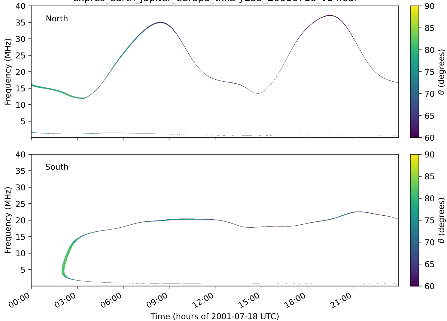
expres_earth_jupiter_europa_txka-y235_20010718_v14.cdf
