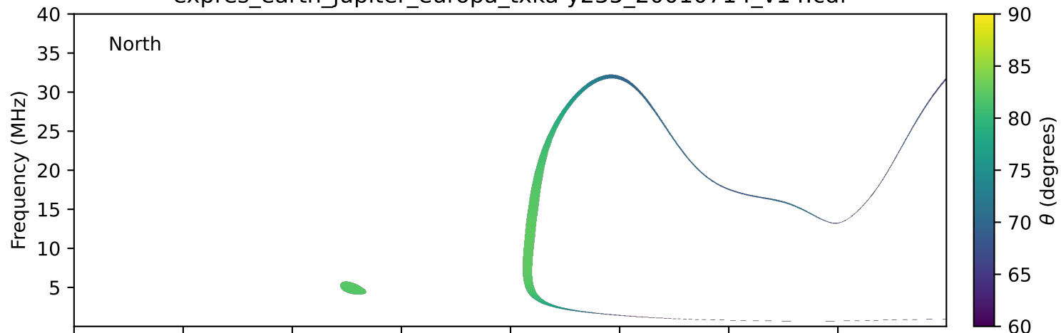
expres_earth_jupiter_europa_txka-y235_20010714_v14.cdf
