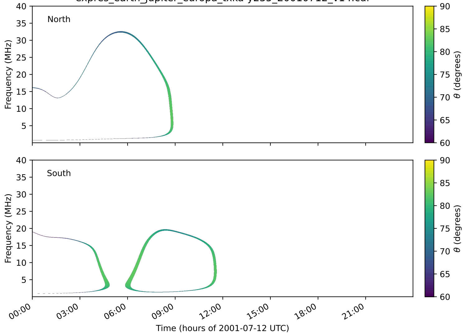
expres_earth_jupiter_europa_txka-y235_20010712_v14.cdf
