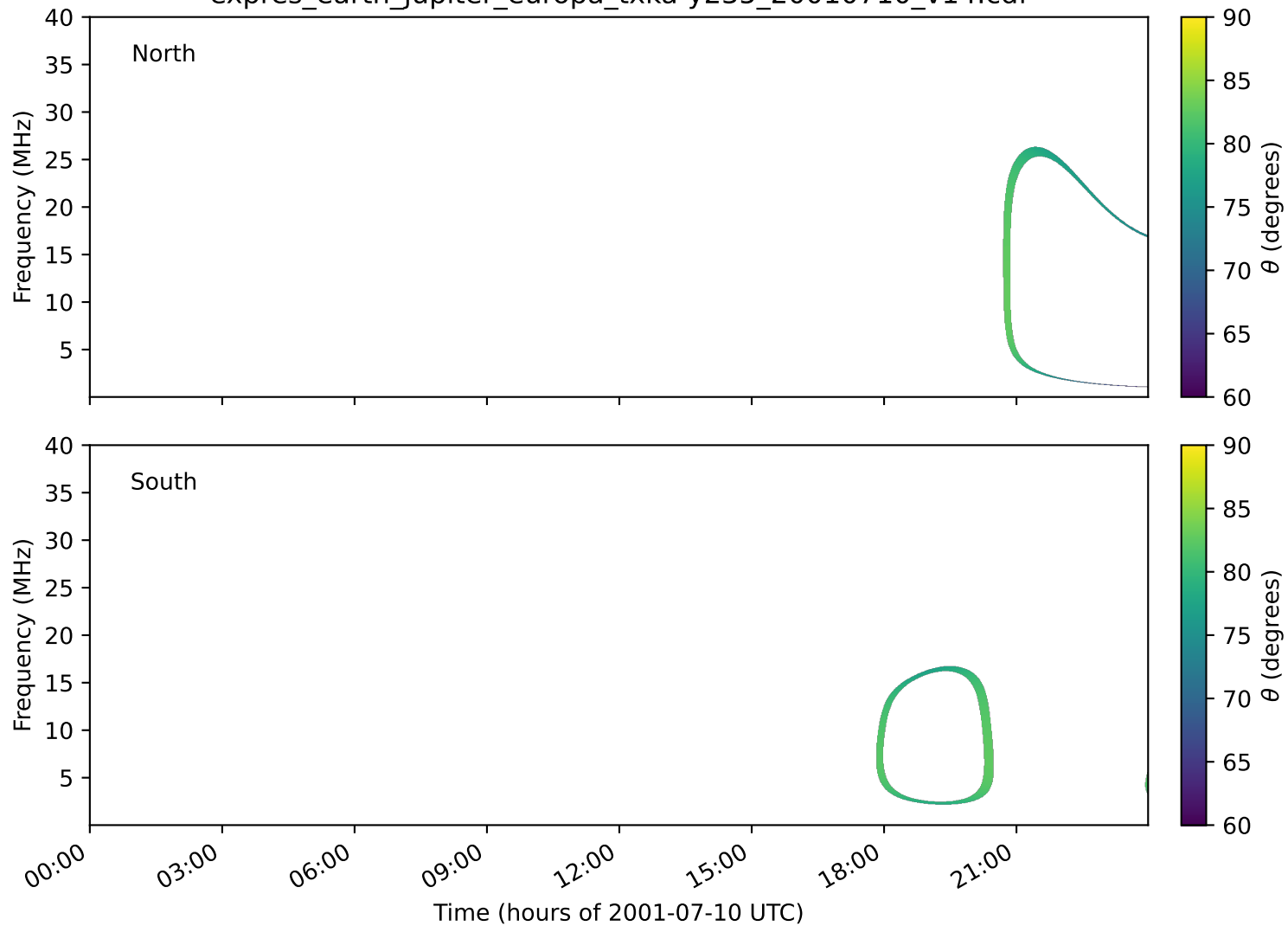
expres_earth_jupiter_europa_txka-y235_20010710_v14.cdf
