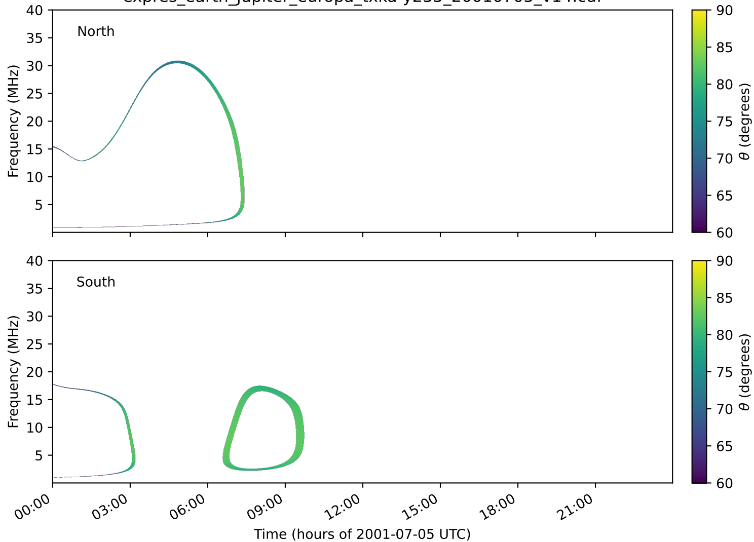
expres_earth_jupiter_europa_txka-y235_20010705_v14.cdf
