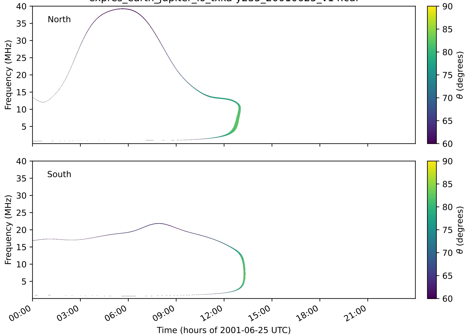
expres_earth_jupiter_io_txka-y235_20010625_v14.cdf
