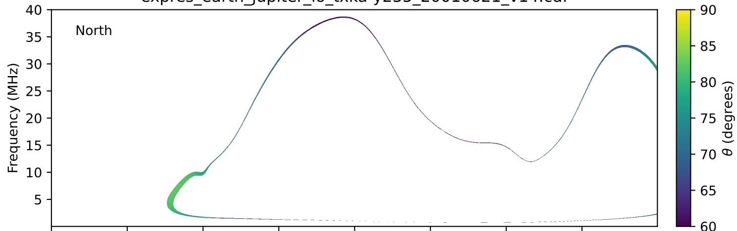
expres_earth_jupiter_io_txka-y235_20010621_v14.cdf
