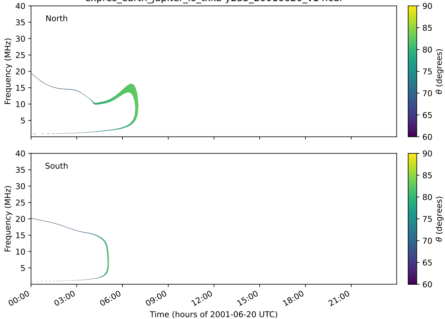
expres_earth_jupiter_io_txka-y235_20010620_v14.cdf
