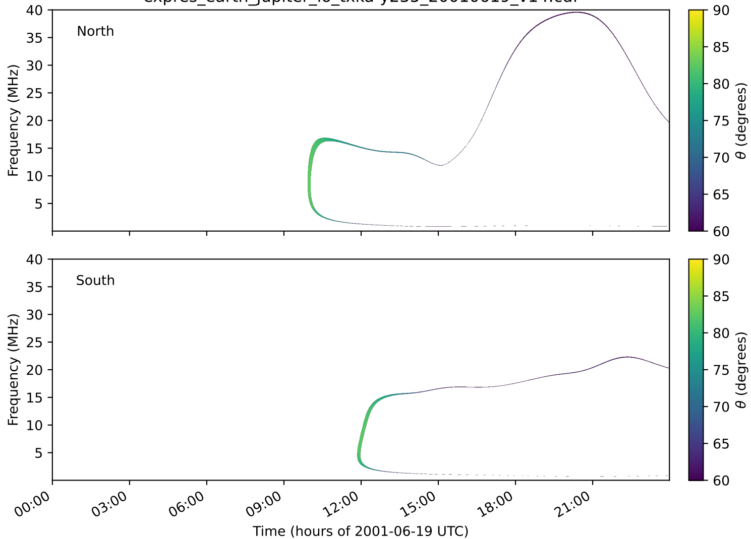
expres_earth_jupiter_io_txka-y235_20010619_v14.cdf
