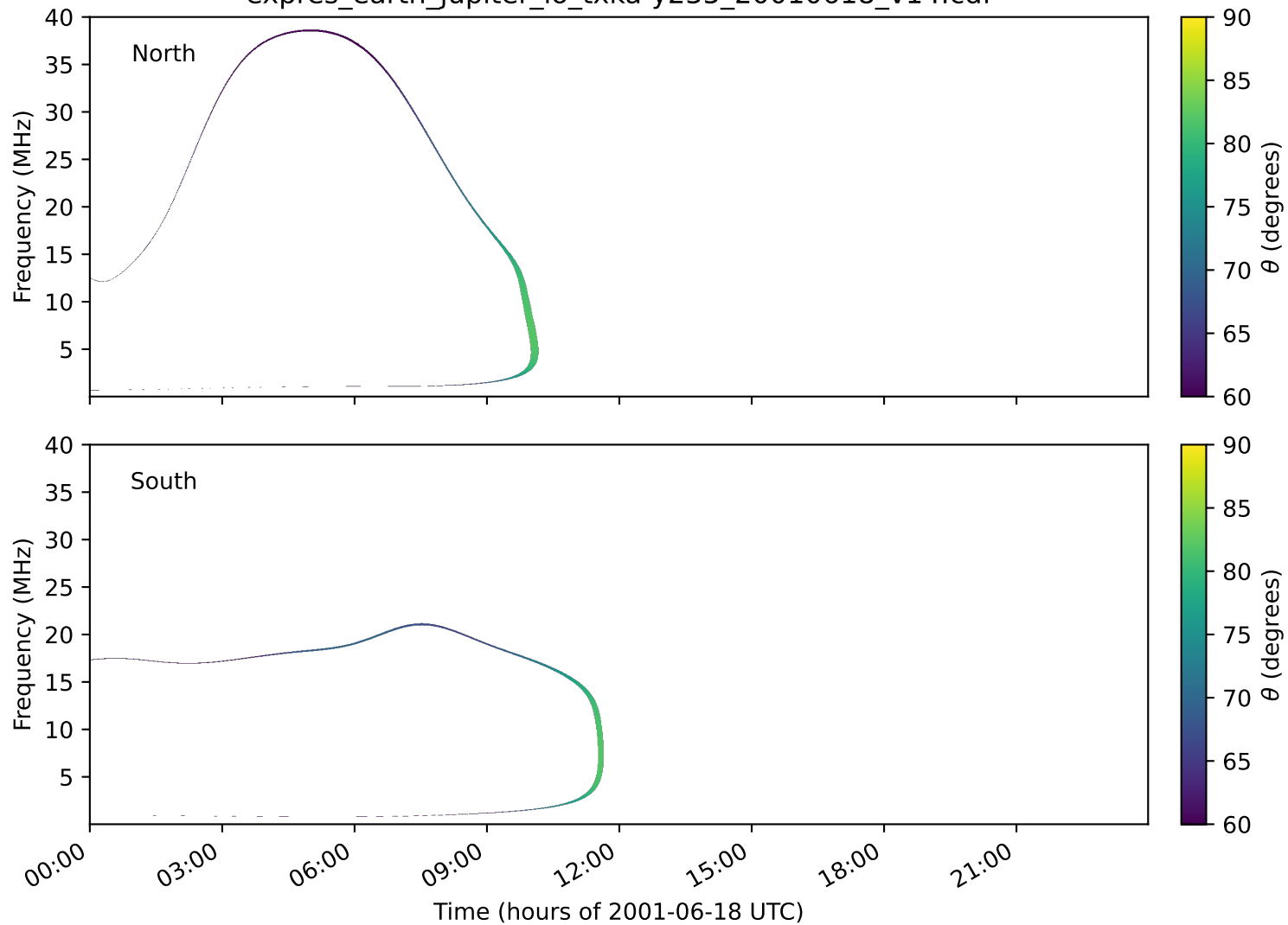
expres_earth_jupiter_io_txka-y235_20010618_v14.cdf
