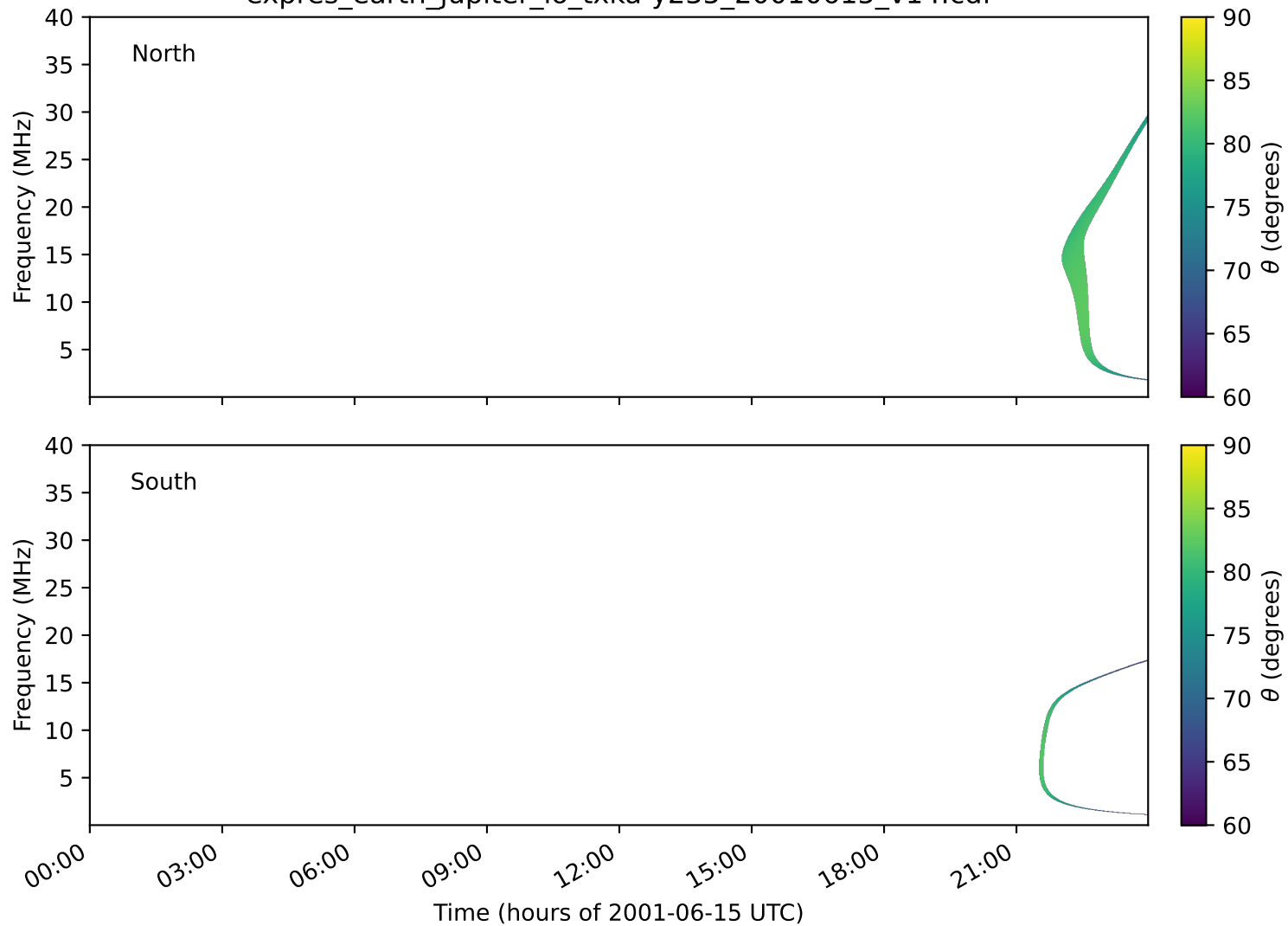
expres_earth_jupiter_io_txka-y235_20010615_v14.cdf
